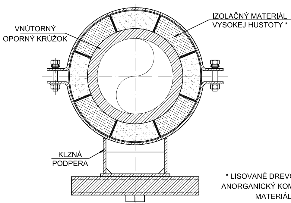
REZ X-X
